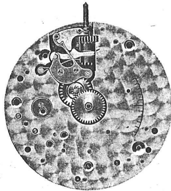
Cal. 433 (16 Size)
